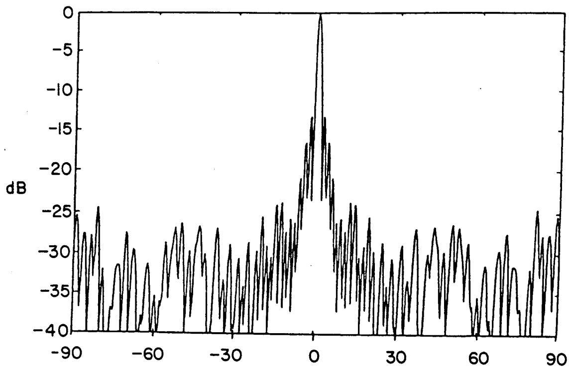
Angle theta in degrees Pattern of a thinned array antenna with randomized spacing containing no grating lobes
