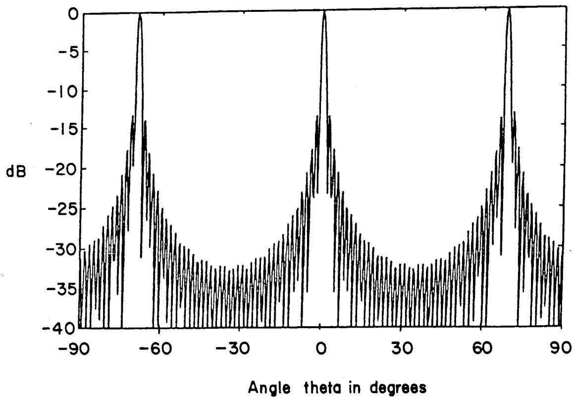
Pattern of a thinned array antenna with uniform spacing containing grating lobes
